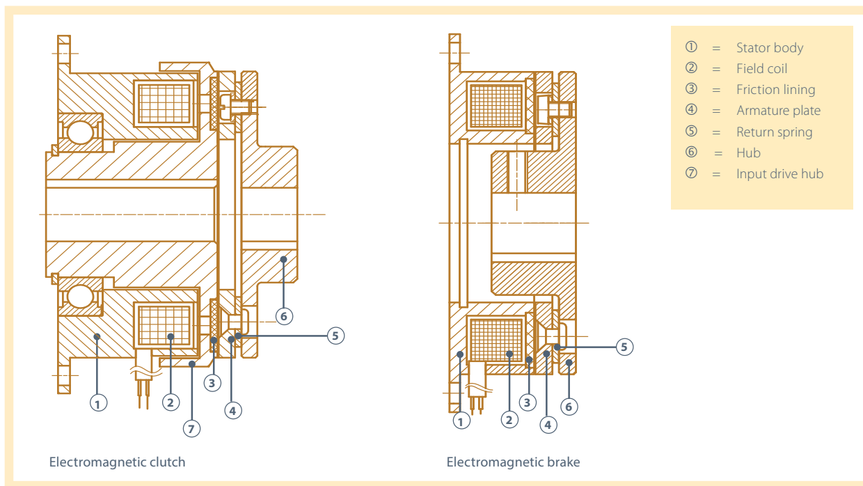
Construction and mode of operation of a electromagnetic clutch /brake
